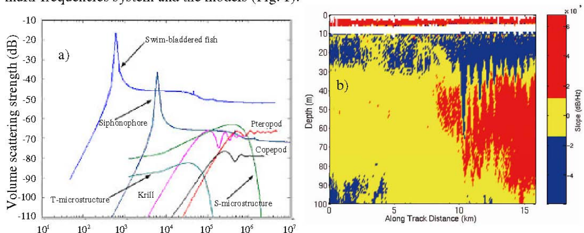
Fig.1 Frequency (Hz): a) The most important biological and physical ocean acoustics scatterers (from [6]) and b) spectral slope (Sv versus frequency) calculated from acoustic-backscatter data at 43, 120, 200, and 420 kHz. The internal wave is divided into distinct regions which have slopes consistent with either biological-scattering processes (red), physical-scattering processes (blue), or both biological-and physical-scattering processes (yellow; from [5])
