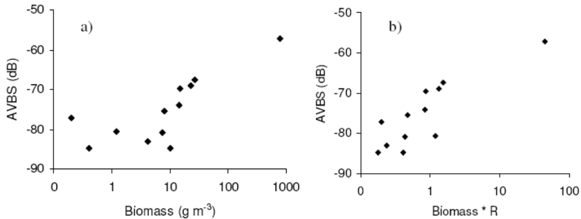
Fig.5 The relationship between volume backscattering (AVBS, 200 kHz) and (a) Nansen biomass ( \text{g m}^{-3} ) and (b) corrected biomass ( \text{g m}^{-3} * R )
