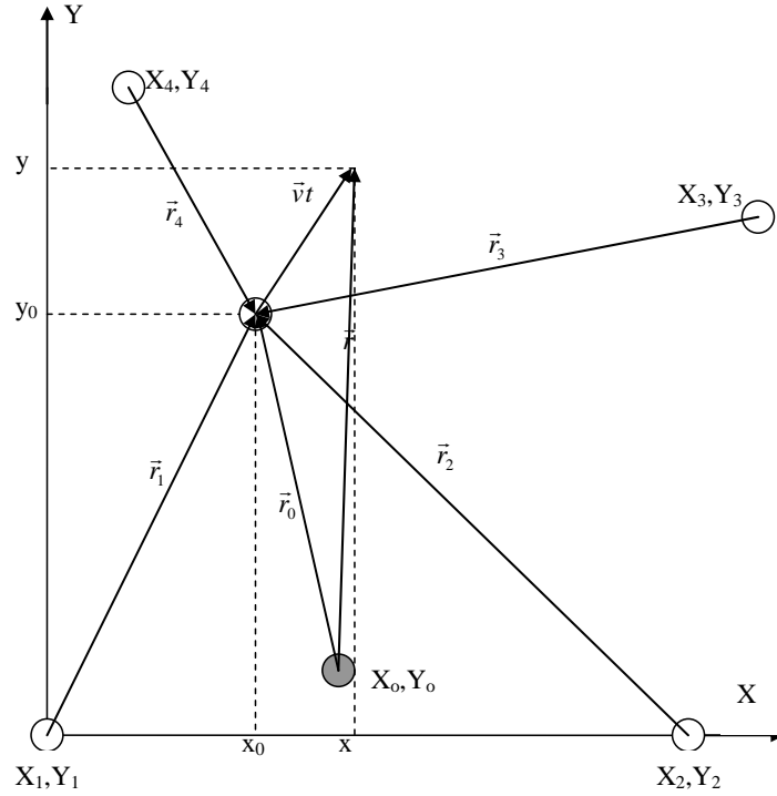
Fig.1. Position of the transmitter (gray), hydrophones and the object under observation in water
